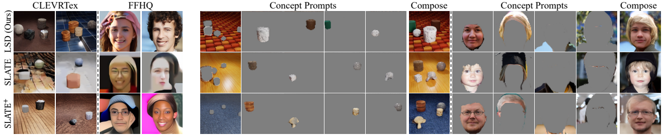
Figure 3. Compositional Image Generation with Concept Prompts. Left: We show some compositional generation samples. LSD provides significantly higher fidelity and clearer details compared to the other methods. Right: We show concept prompts constructed by composing arbitrary slots from our visual concept library and the corresponding generated image by LSD.
