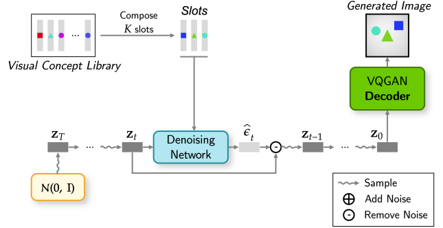
Figure 1. Compositional Image Generation. Given the trained model, we can generate novel images by composing a slot-based concept prompt and decoding it using the trained latent slot diffusion decoder.
