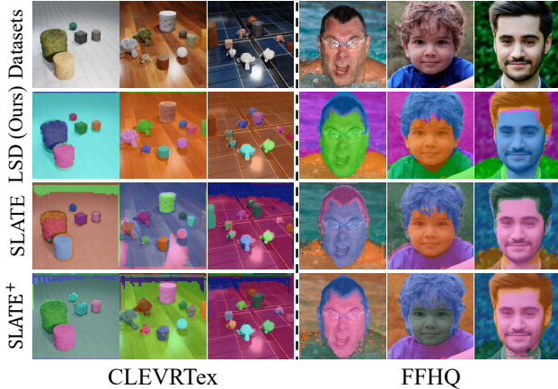
Figure 2. Visualization of Unsupervised Object Segmentation. We show visualizations of predicted segments on CLEVRTex and FFHQ datasets.
