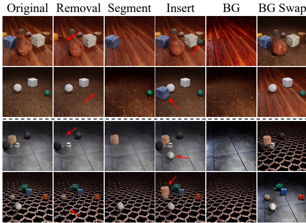
Figure 4. Slot-Based Object Manipulation. We show the slot-based image editing ability of our model. In particular, we show edit operations such as object removal, object extraction, object insertion, background extraction, and background swapping.
